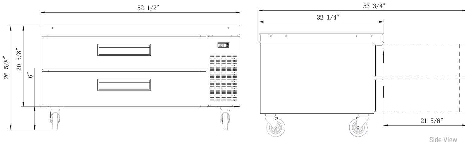
Side View
