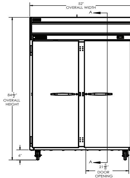
ELEVATION VIEW
